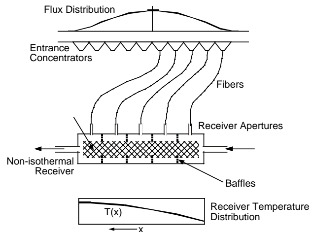
Figure 1. Fiber distributor and non-isothermal receiver for concentrated solar energy. Top: non-uniform flux distribution incident on the target of the primary collector. Bottom: temperature distribution along the receiver.
