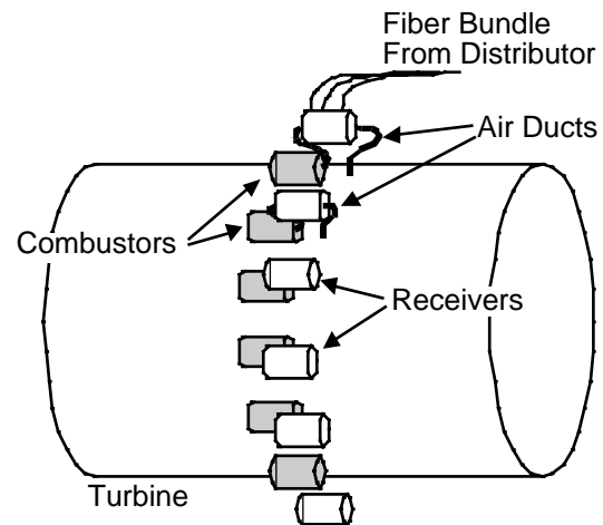
Figure 2. Distributed receiver system for a gas turbine with a distributed annular combustor. Each combustor is preceded with a separate receiver, and each receiver is supplied with a separate fiber bundle.
