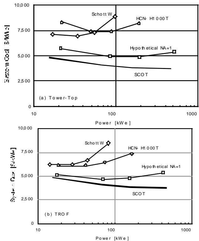
Figure 5. Plant specific cost of (a) the Tower-Top and (b) the TROF systems, compared to the non-fiber SCOT system, as a function of plant rated power. The results are shown for the three types of fibers.
