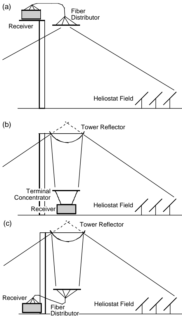
Figure 3. Three system designs: (a) Tower-top, (b) SCOT, and (c) TROF.
