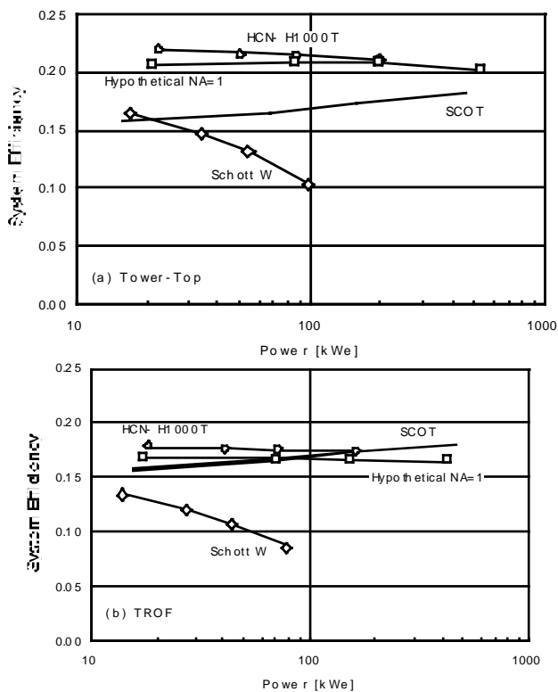
Figure 4. Overall conversion efficiency of (a) the Tower-Top and (b) the TROF systems, compared to the non-fiber SCOT system, as a function of plant rated power. The results are shown for the three types of fibers.
